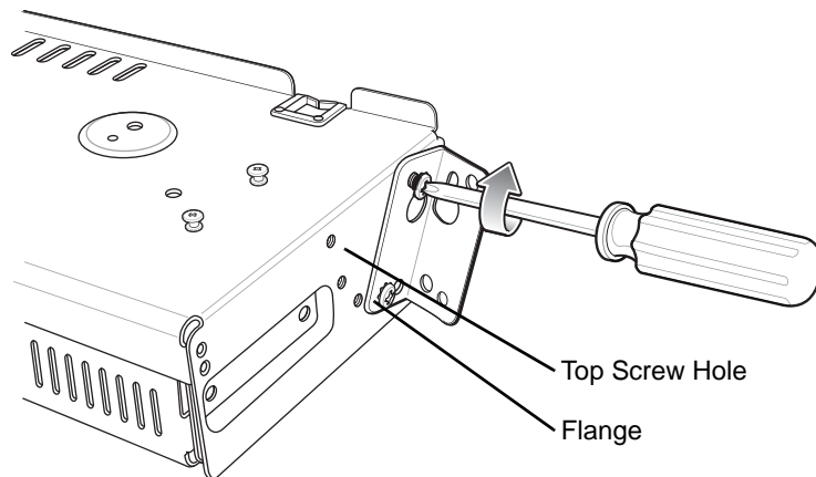
Figure 2-33 Flange 25° Position (4-Slot Battery Chargers)
