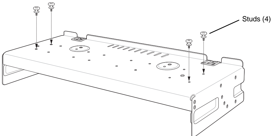
Figure 2-20 Install Studs
