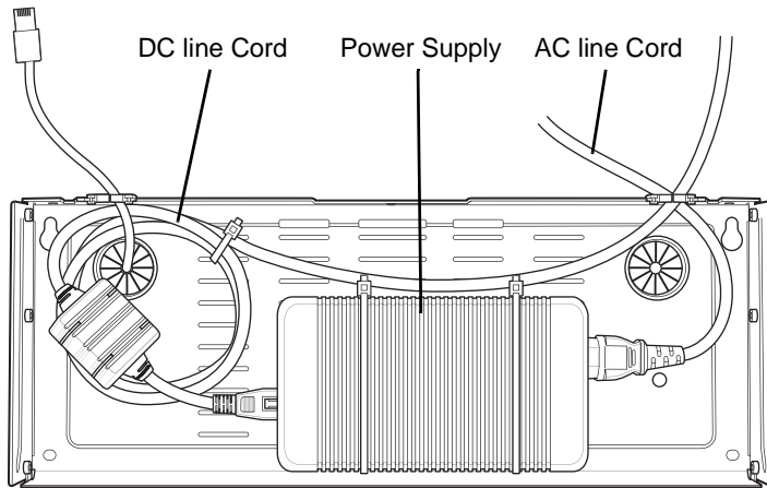
Figure 2-19 Power Supply in Bottom Tray
