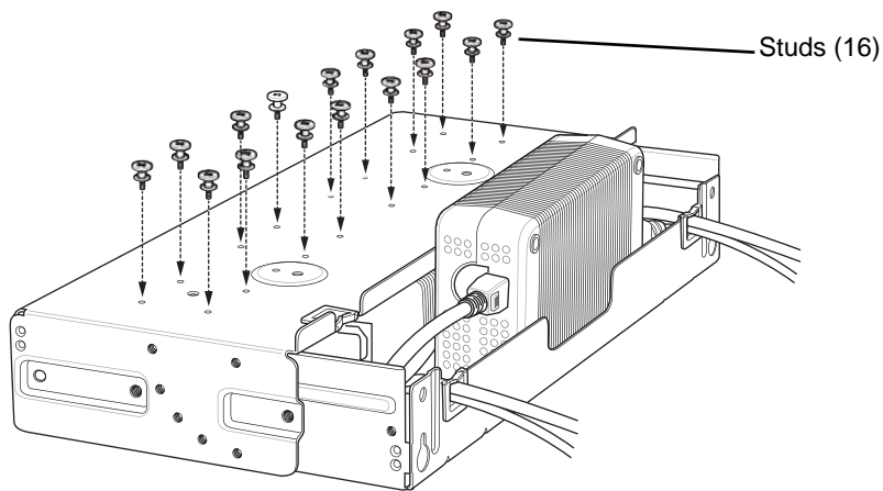
Figure 2-28 Install Studs
