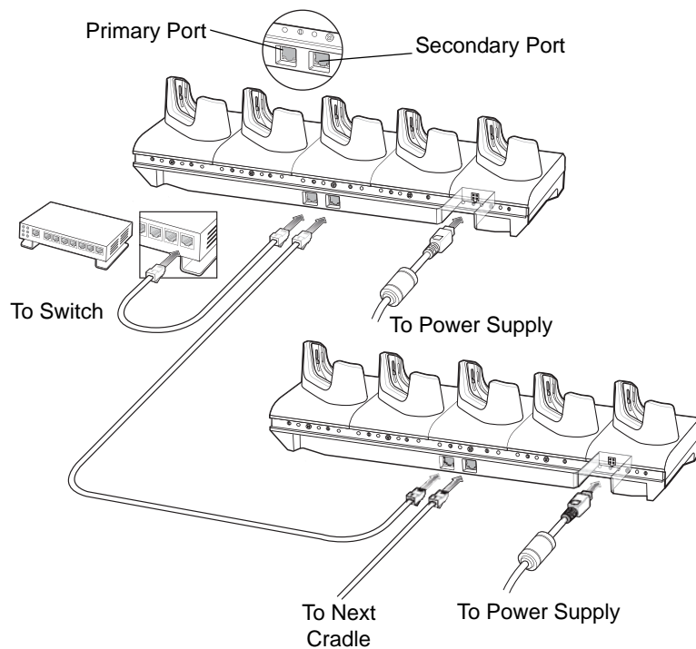
Figure 2-12 Daisy-chaining 5-Slot Ethernet Cradles
