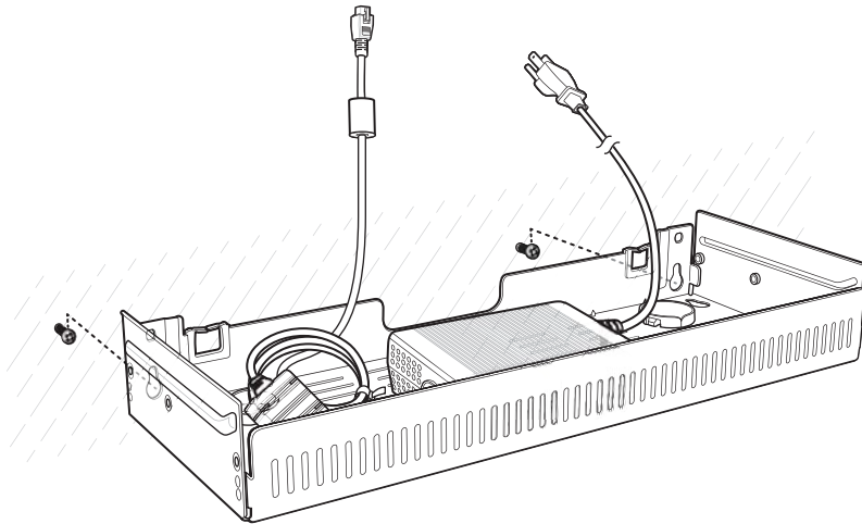
Figure 2-37 Horizontal Installation
