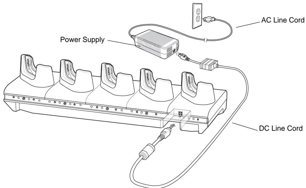
Figure 2-8 5-Slot Charge Only Cradle Setup
