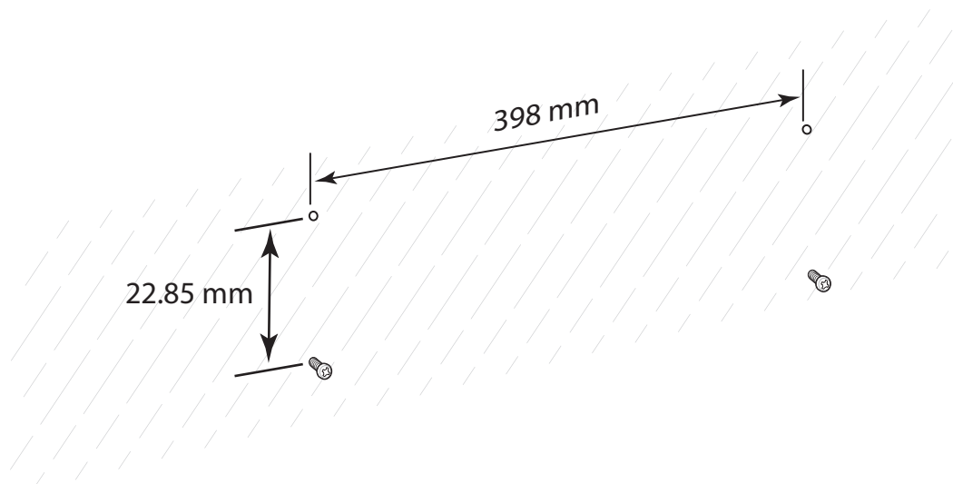
Figure 2-36 Horizontal Mounting Template
