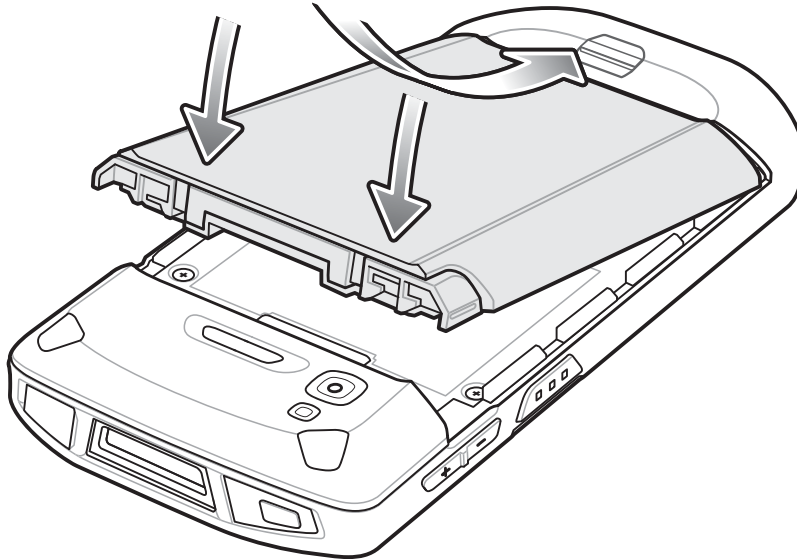
Figure 1-7 Insert Bottom of Battery into Battery Compartment
