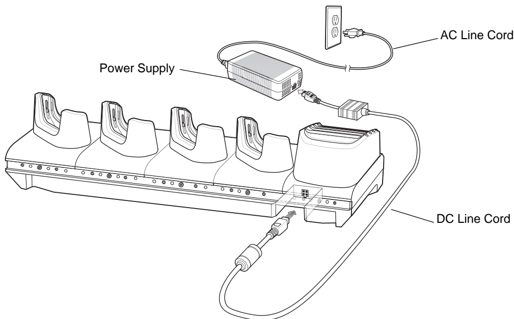
Figure 2-4 4-Slot Charge Only Cradle with Battery Charger Setup
