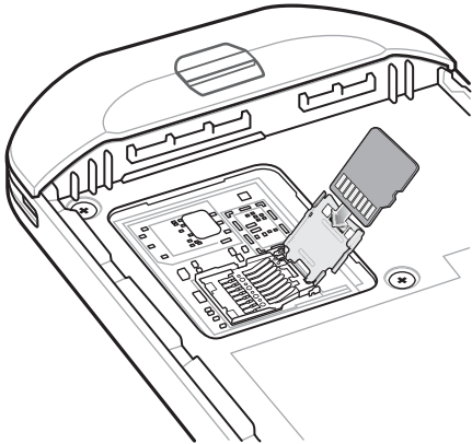
Figure 1-4 Insert microSD Card in Holder
