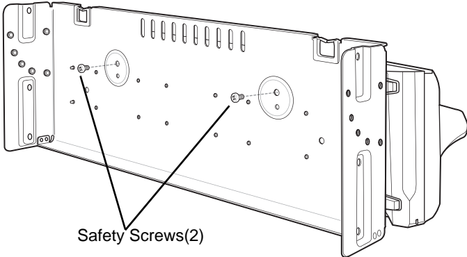
Figure 2-22 Secure Cradle
