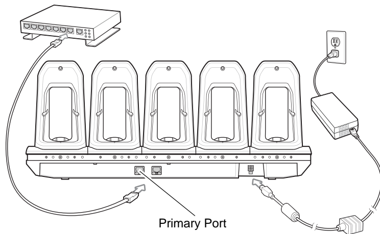
Figure 2-11 5-Slot Ethernet Cradle Setup
